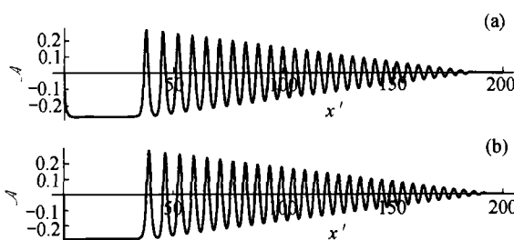
Fig. 1. Numerical (a) and theoretical (b) results of tailing wavetrain generation
